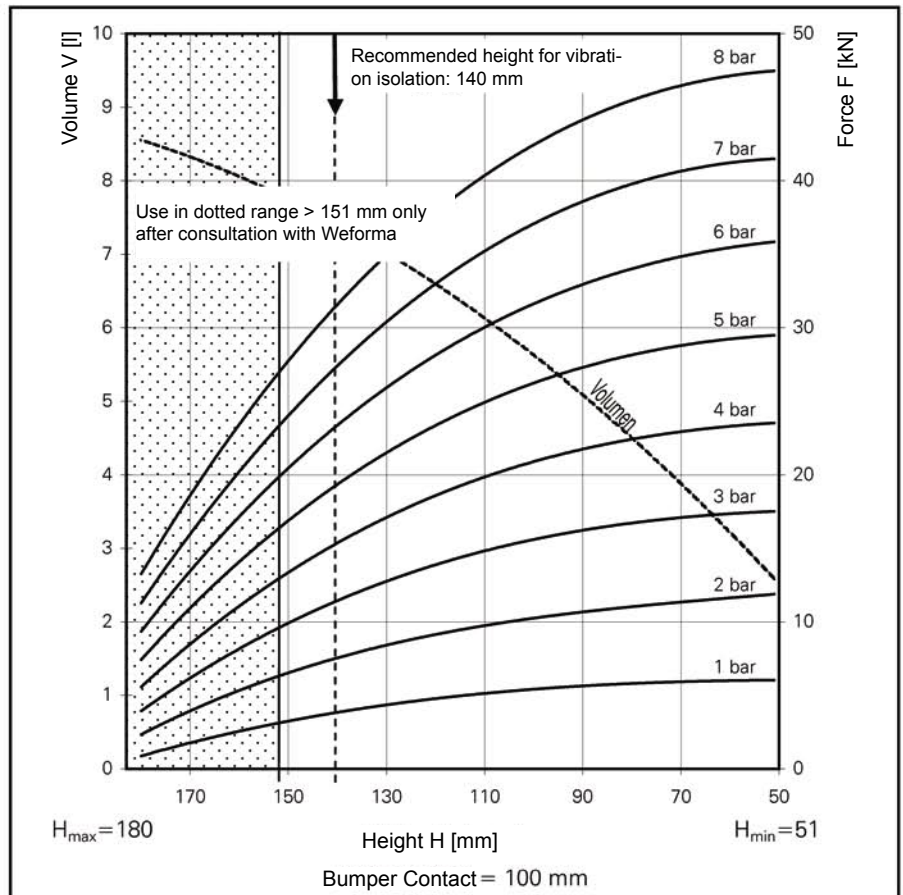
Force-height diagramm
